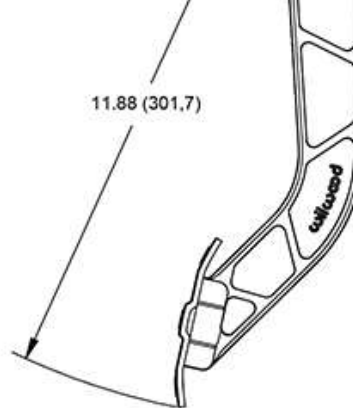
FOOT PAD DETAIL
